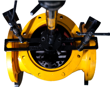
Flat Bar Clamping mounted on valve body
